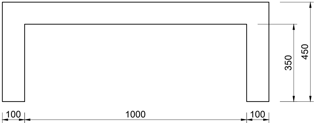
FRONT ELEVATION
